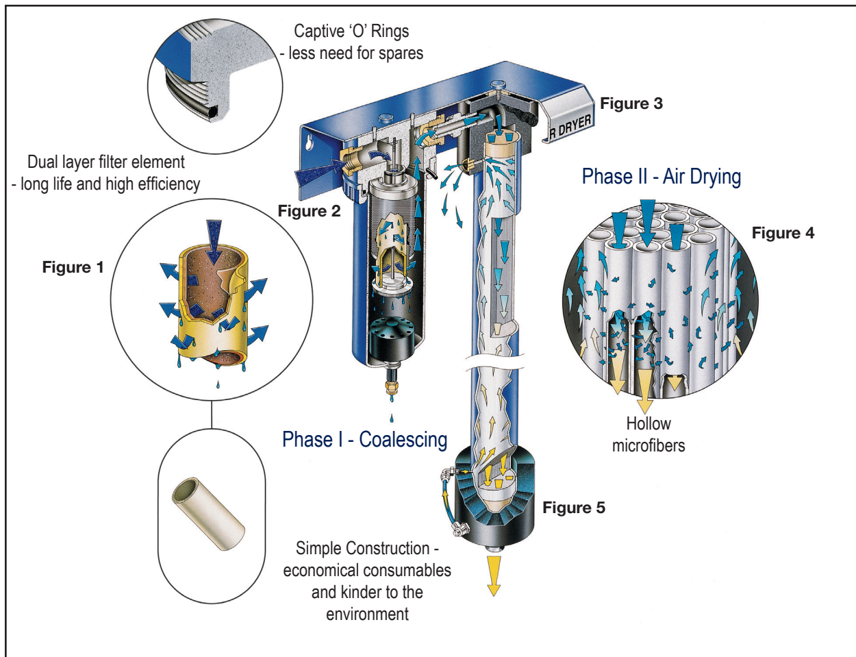
Membrane Air Dryer - Principal of Operation
